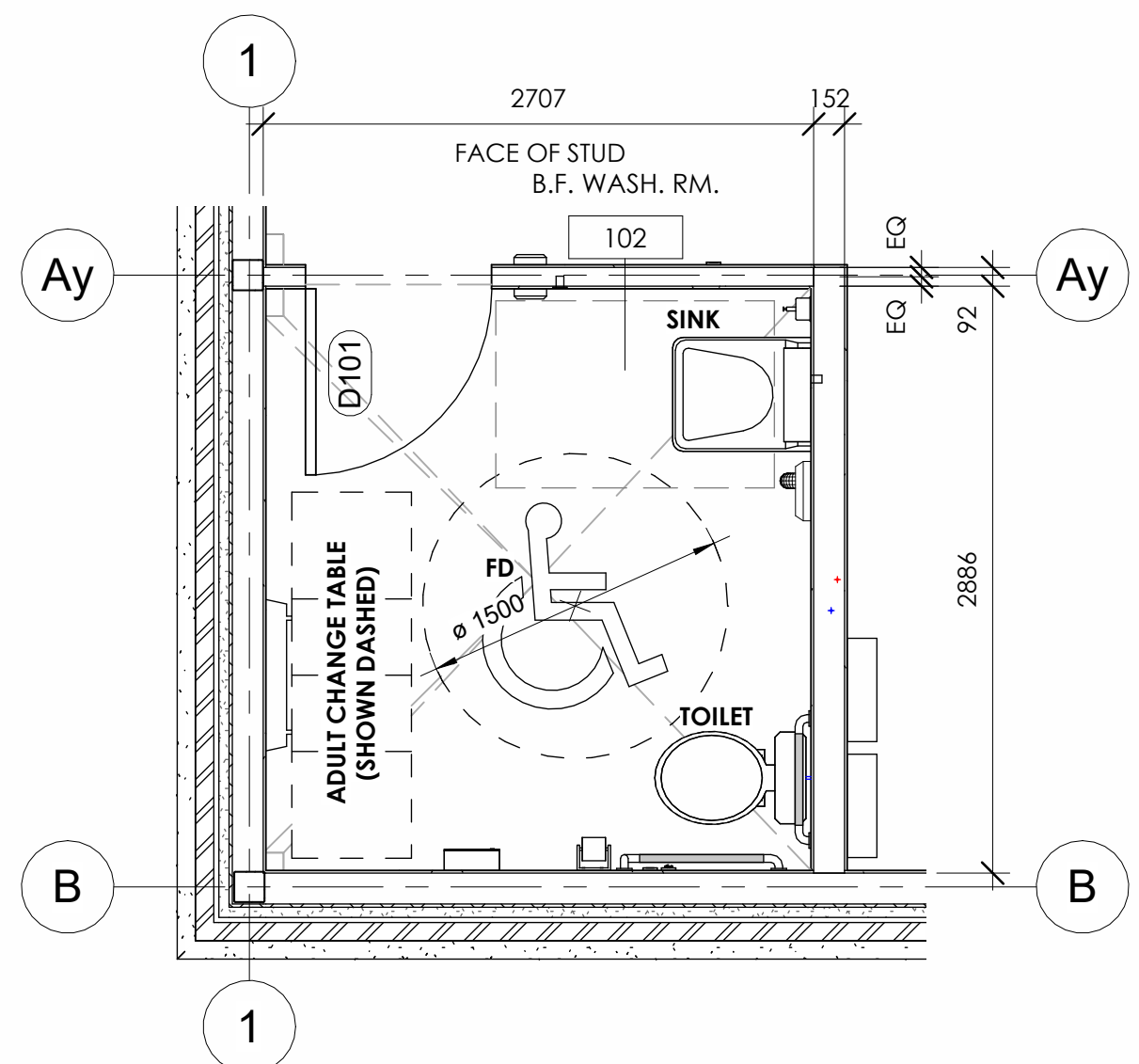
4 Enlarged B.F. Washroom Plan 1:35
