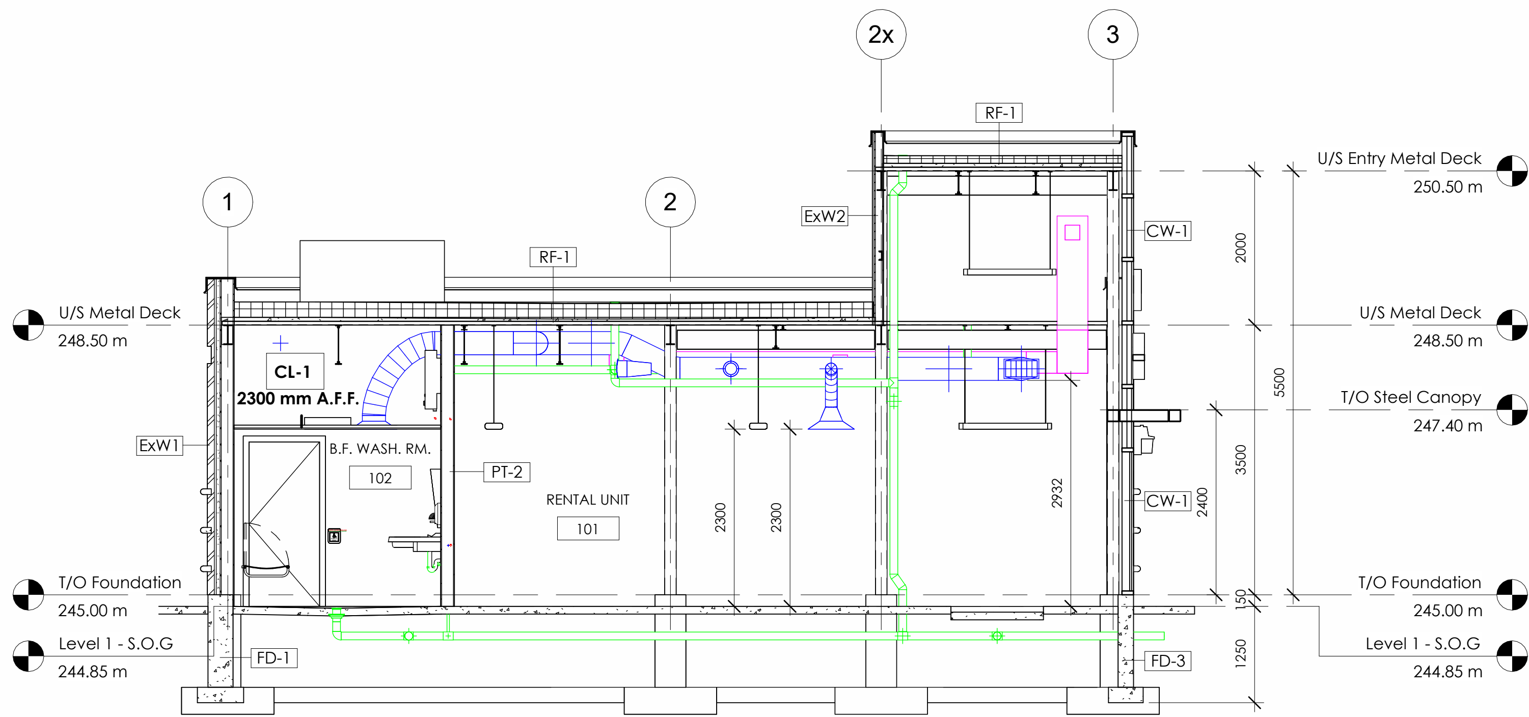
2 EAST-WEST BUILDING SECTION 1:50
