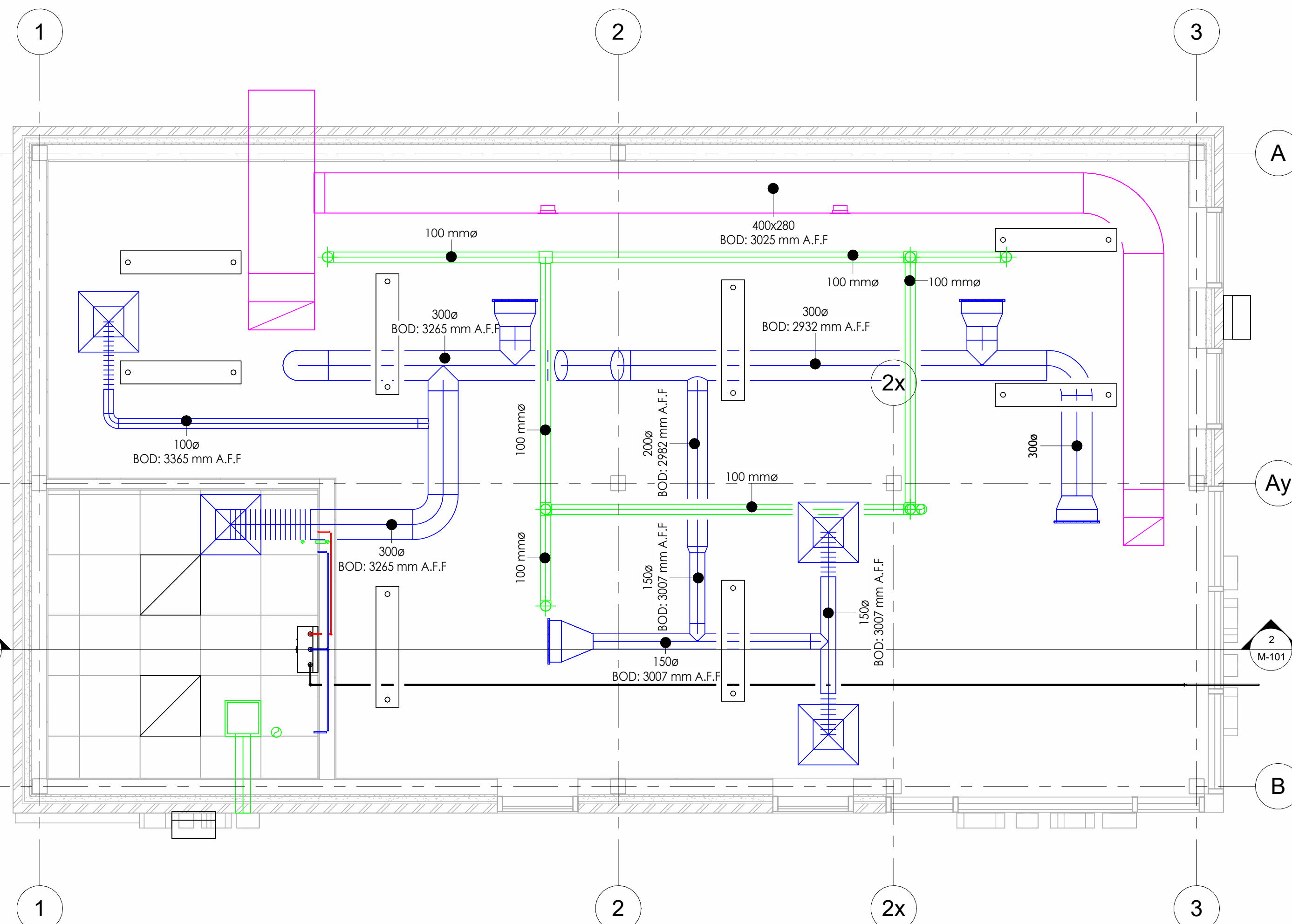
4 SYSTEMS R.C.P. 1 : 35
