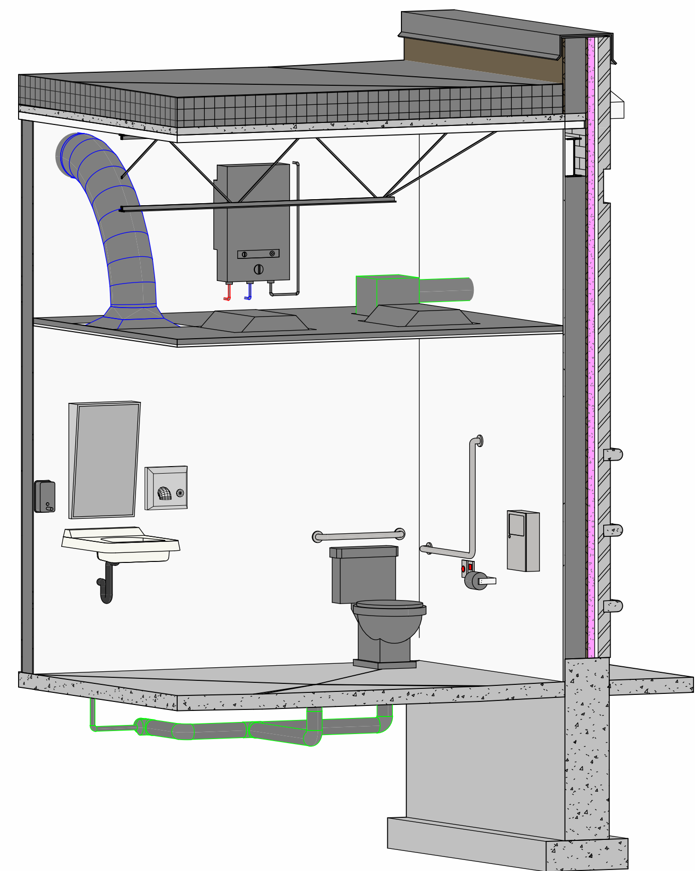
5 B.F. WASHROOM ISOMETRIC
