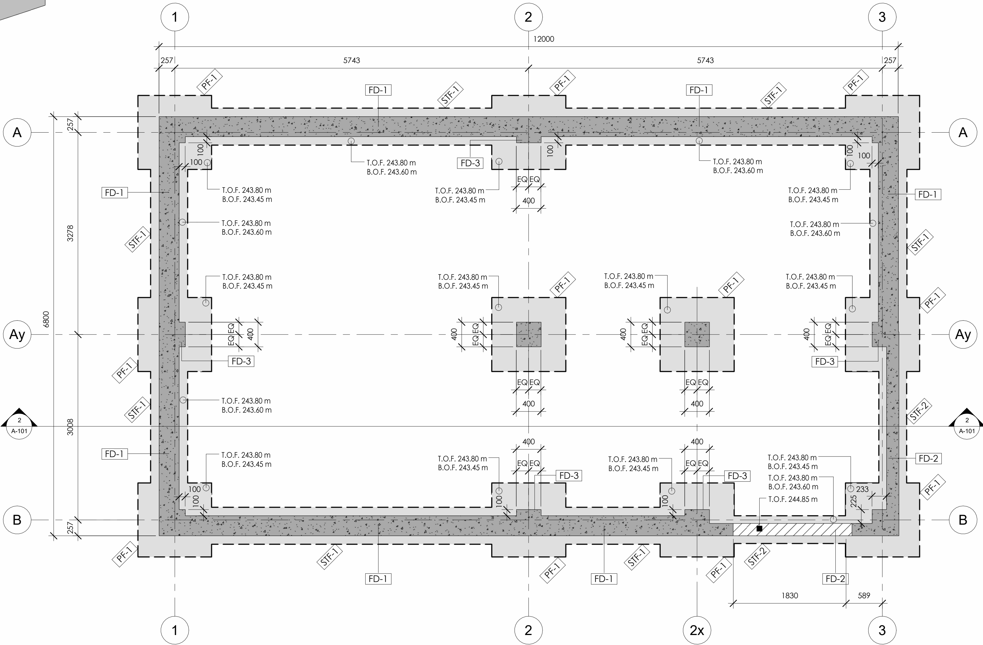
1 FOUNDATION PLAN
