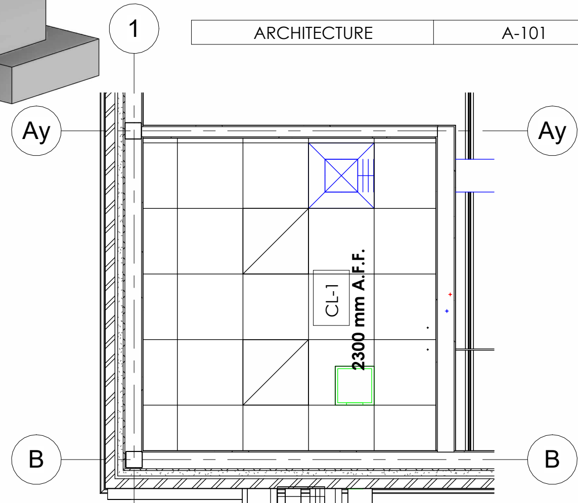
3 WASH. ROOM R.C.P. 1:35
